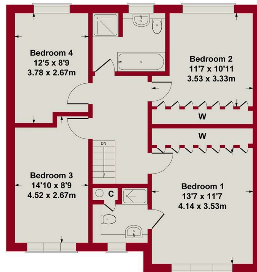
FIRST FLOOR
